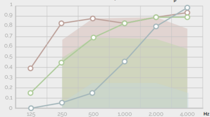
Practical sound absorption coefficient, \alpha_p
