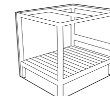
103.1956 (205x175x200 cm) 103.1957 (205x155x200 cm) 103.1958 (205x205x200 cm)
