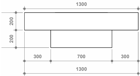
Vista Frontal
