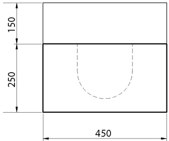
Vista Frontal
